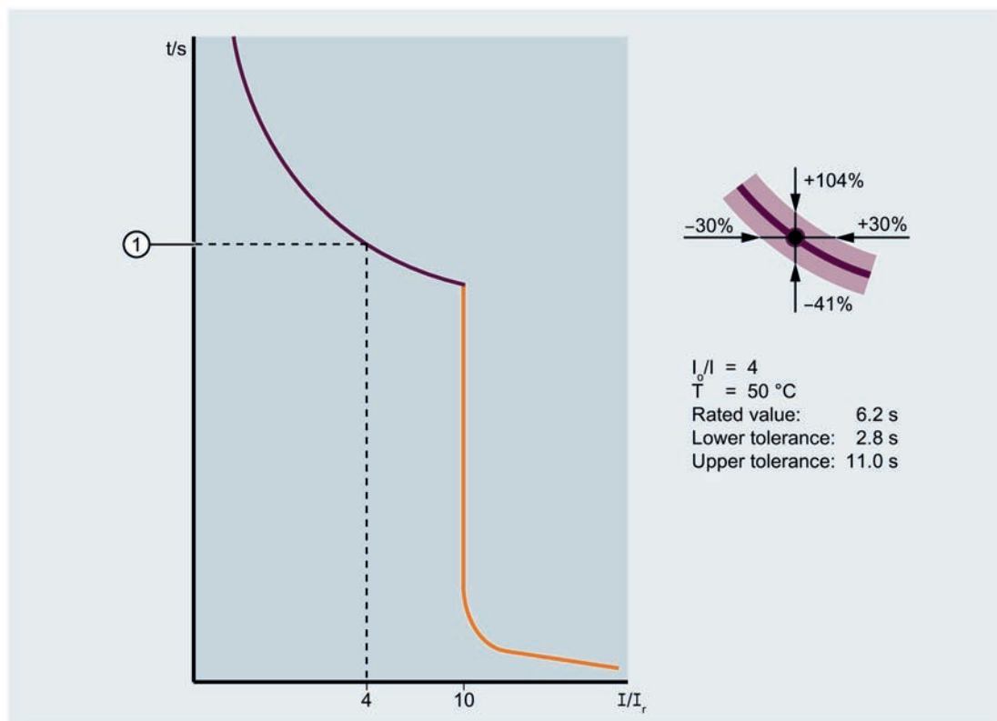
① Tripping time (schematic representation)
