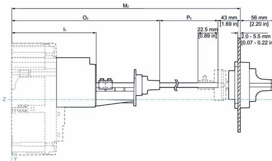
Supplementary handle for door mounted rotary operator 3VA9.87 - 0GA80
