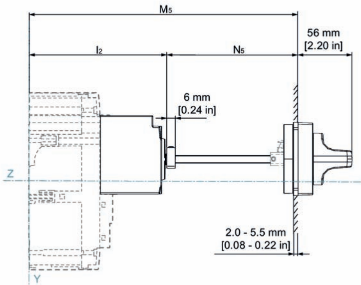
Door mounted rotary operator for 3VA up to 630 A (3VA9..7 - 0FK61)
