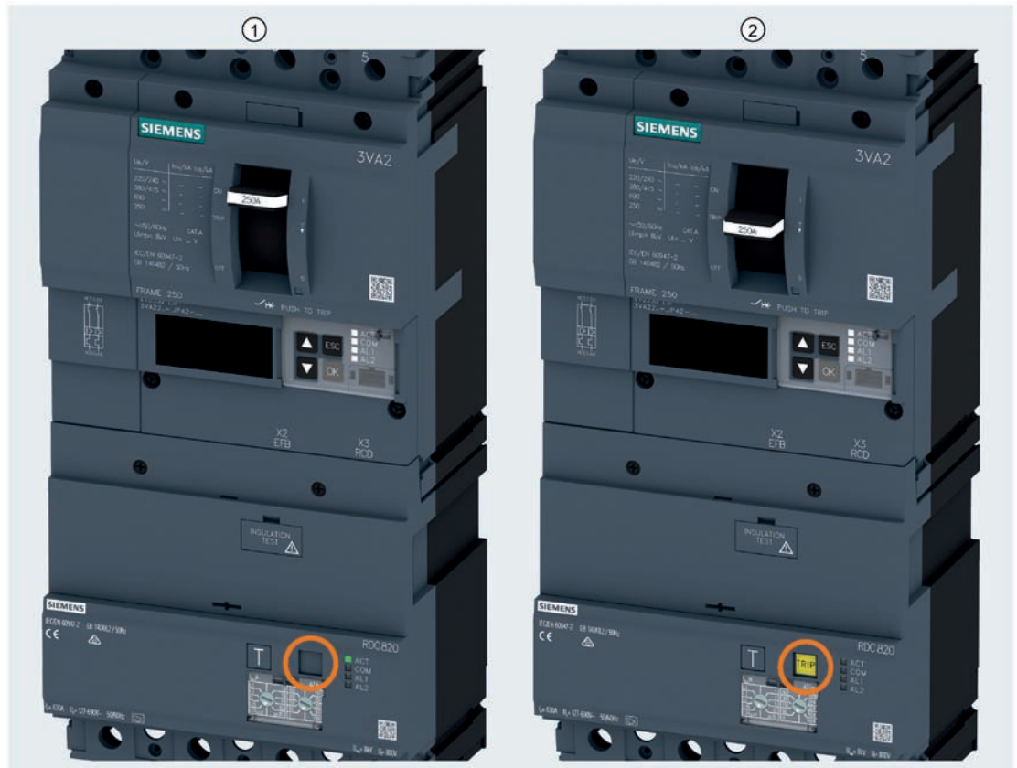
① Residual current device is operating normally and has not tripped
